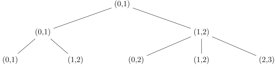
Figure 3: Ascent sequences a of length at most 3 relabeled with the pair (p, q)
